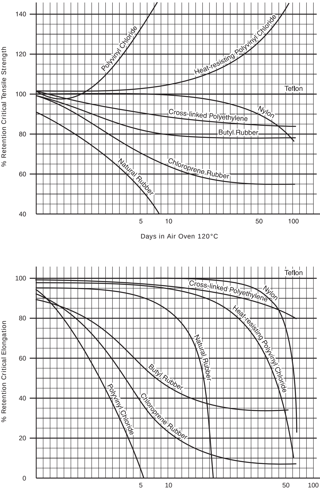
LONG-TIME HEAT AGING CURVES
